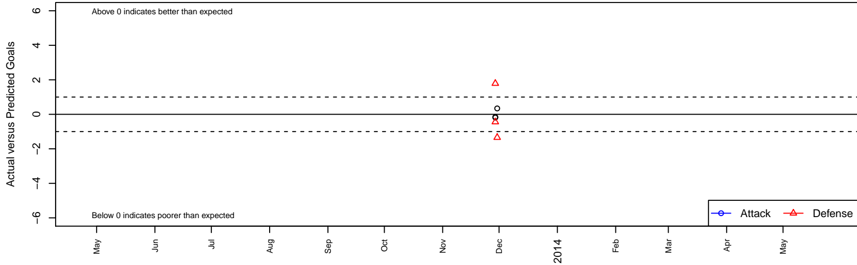
Rebels SC G02 Dots are actual minus expected GF (blue circles) and GA (red triangles). Blue line is smoothed change in attack strength. Red is smoothed change in defense strength.
